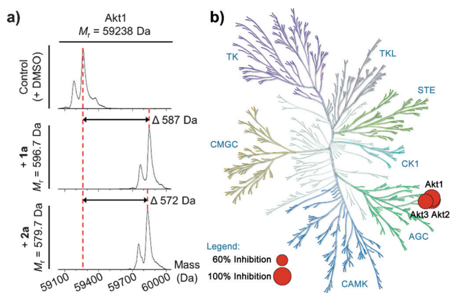
Figure 2. a) Deconvoluted mass spectra of Akt1 incubated with DMSO (top), 1a (middle), and 2a (bottom), respectively. Mass differences in relation to DMSO-treated control are displayed as \Delta values and demonstrate covalent modification of Akt1 with 1a and 2a . b) Kinome dendrogram of 1a . At 1 \mu M compound concentration, only Akt1, Akt2, and Akt3 were significantly inhibited (98%, 96%, and 83%) whereas the remaining 97 kinases were inhibited by less than 40%. Kinase profiling data were generated with the SelectScreen Profiling Service from Life Technologies. The kinase dendrogram was adapted from Kinome Render [22] and the illustration is reproduced with courtesy of Cell Signaling Technology, Inc. ( http://www.cellsignal.com ).
